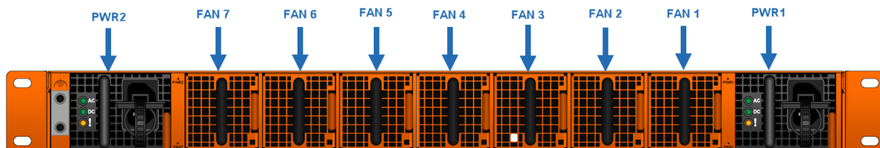
GigaVUE-TA400 Rear View
